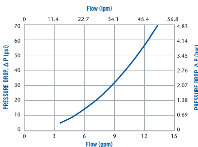
CQHD06 WATER FLOW
