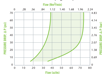
DPC AIR FLOW • 100 psig inlet pressure
